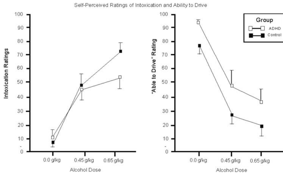
Figure 4. Mean self-perceived ratings of intoxication and ability to drive for the control and ADHD groups under three alcohol doses: 0.0g/kg (placebo), 0.45g/kg, and 0.65g/kg. Capped vertical lines show standard errors of the mean.
