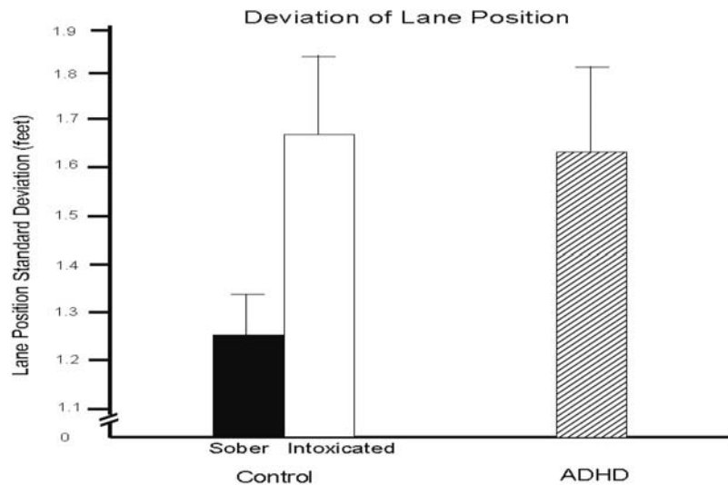
Figure 1. Mean within-lane deviation for the control group while sober and intoxicated and for the ADHD group. Capped vertical lines show standard errors of the mean.
