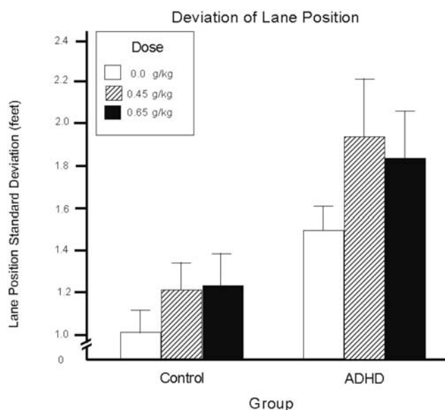
Figure 2. Mean within-lane deviation for the control and ADHD groups under three alcohol doses: 0.0g/kg (placebo), 0.45g/kg, and 0.65g/kg. Capped vertical lines show standard errors of the mean.
