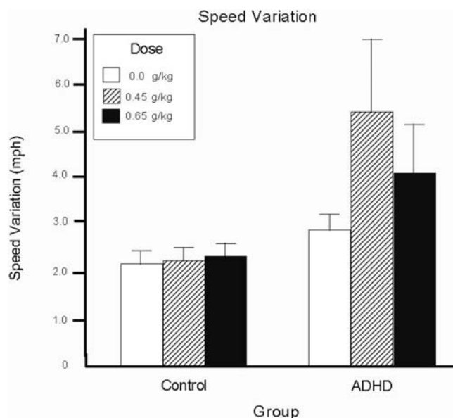
Figure 3. Mean speed variation for the control and ADHD groups under three alcohol doses: 0.0g/kg (placebo), 0.45g/kg, and 0.65g/kg. Capped vertical lines show standard errors of the mean.
